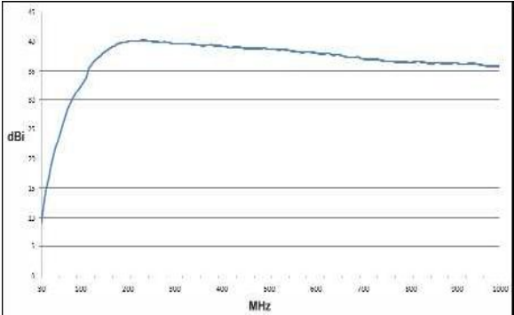
Gain Diagram BicoLOG 30100EX
