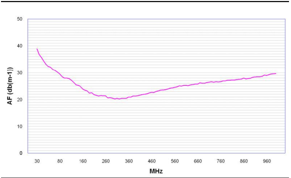
Antenna factor BicoLOG 30100EX
