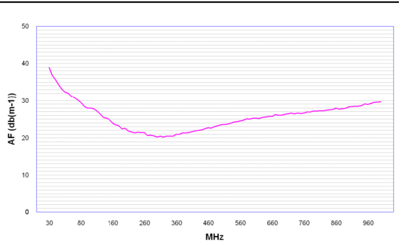
Antenna factor BicoLOG 30100X
