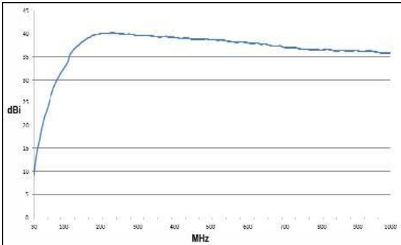
Gain Diagram BicoLOG 30100X
