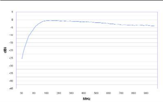
Gain Diagram BicoLOG 30100E
