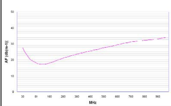
Antenna factor BicoLOG 30100E
