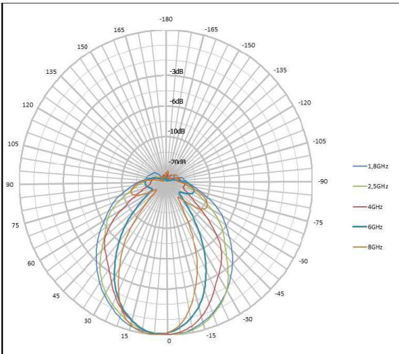
Vertical Pattern (typical) HyperLOG 70xx Series
