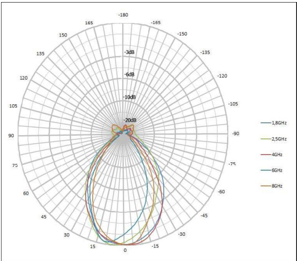
Horizontal Pattern (typical) HyperLOG 70xx Series
