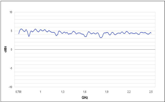
Gain Diagram HyperLOG 7040
