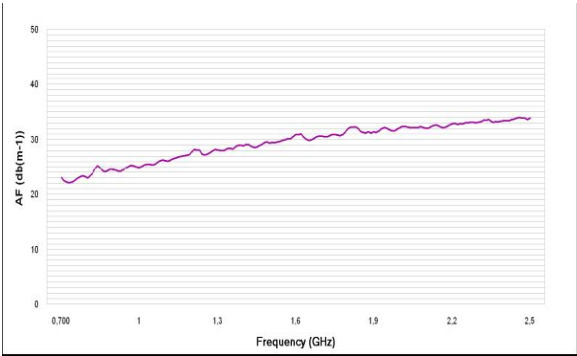
Antenna factor HyperLOG 7040
