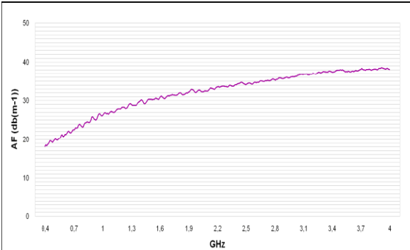
Antenna factor HyperLOG 4040
