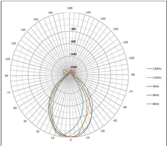
Gain Diagram HyperLOG 4040
